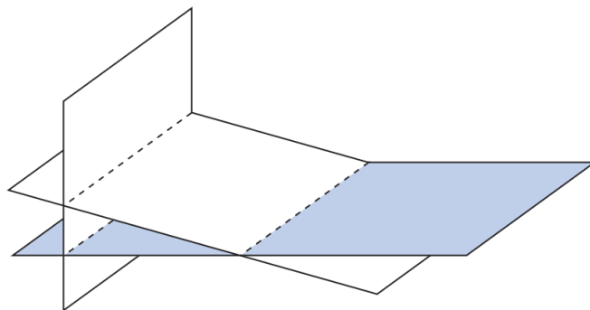
Figure 2(b) Three planes with no common intersection.
